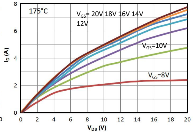
Fig 2: Output Characteristics
